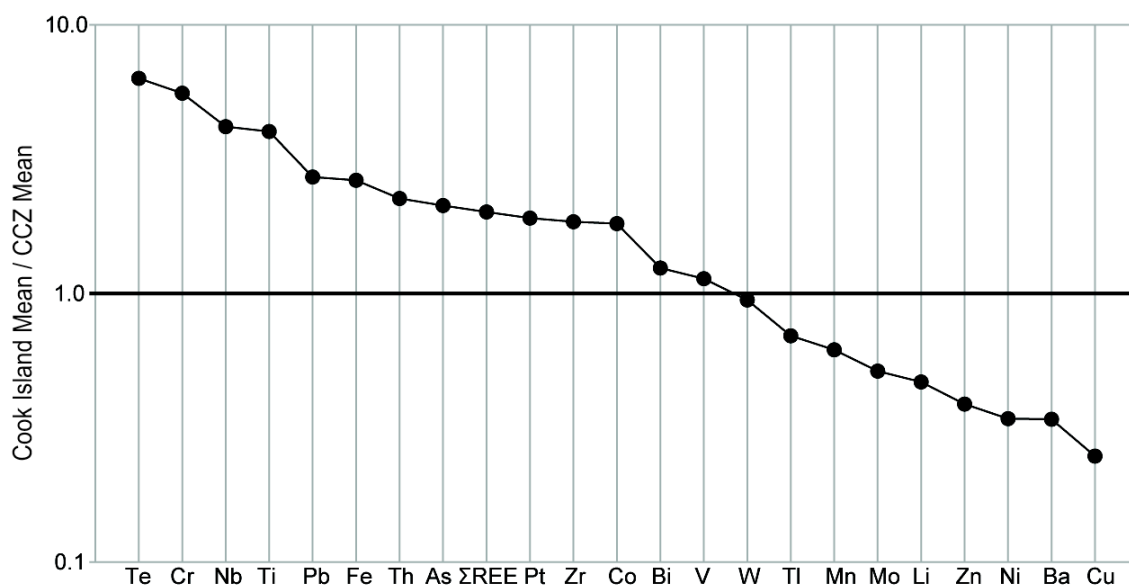
Figure 1. Comparison of Cook Islands (CI) nodule grades with those from the Clarion-Clipperton Zone (CCZ) nodules. Metals above the 1.0 line are enriched in CI nodules and those below the line are enriched in CCZ nodules.
