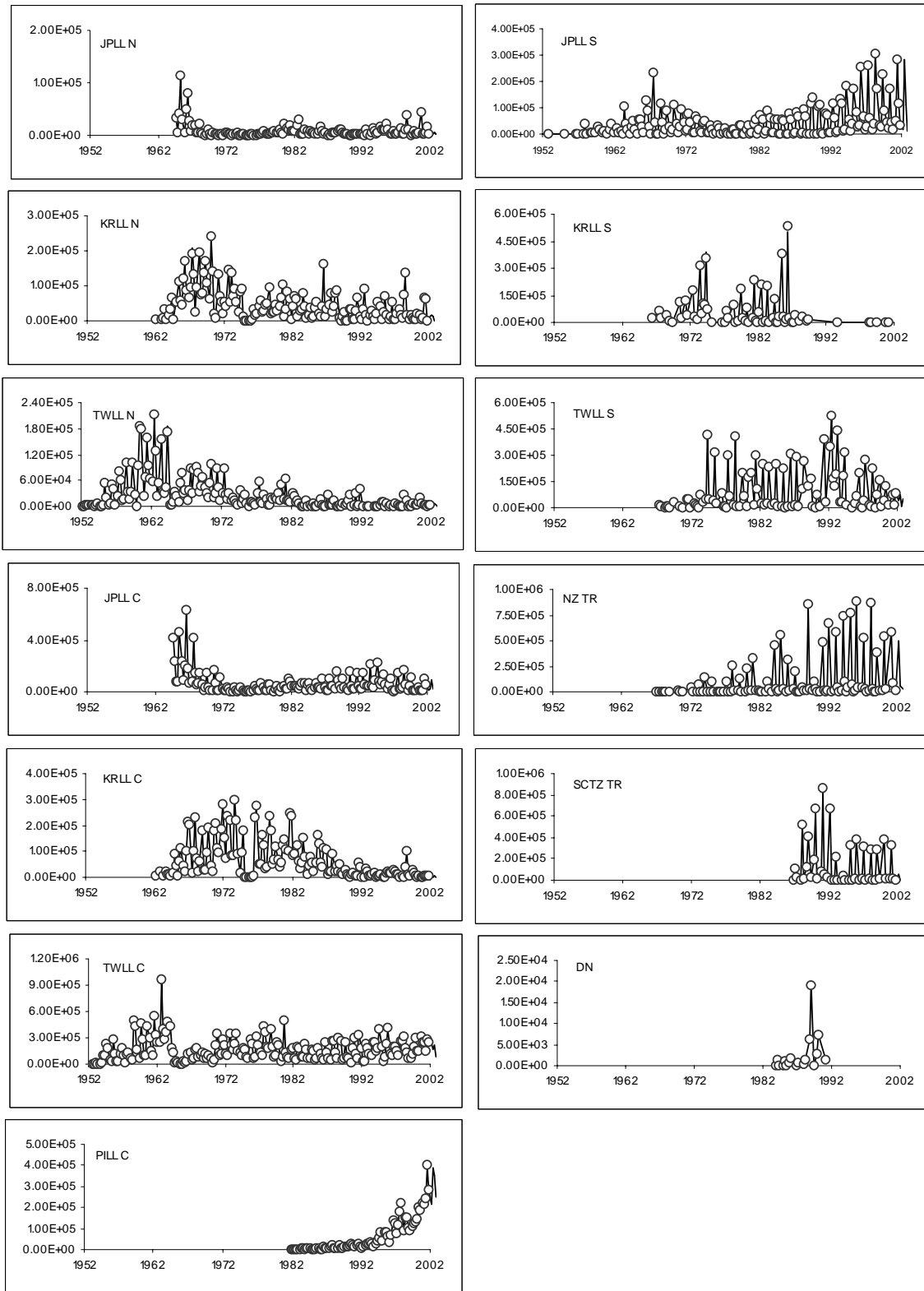
Figure 5. Observed (circles) and predicted (lines) total catches by fishery and quarter. Catches are in number for all fisheries except the driftnet (DN) fishery, where the catches are in tonnes.
