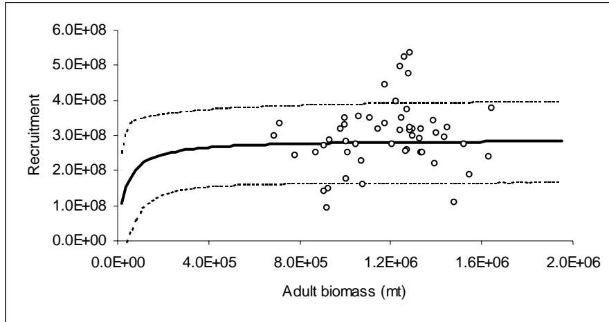
Figure 19. Spawning biomass – recruitment estimates and the fitted Beverton and Holt stock-recruitment relationship (SRR) incorporating a prior on steepness of 0.9. The dashed lines are the 95% confidence intervals on the SRR.
