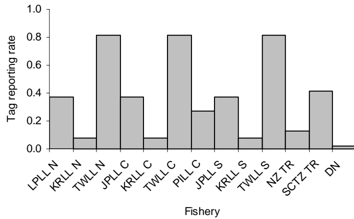
Figure 9. Estimated tag-reporting rates by fishery.
