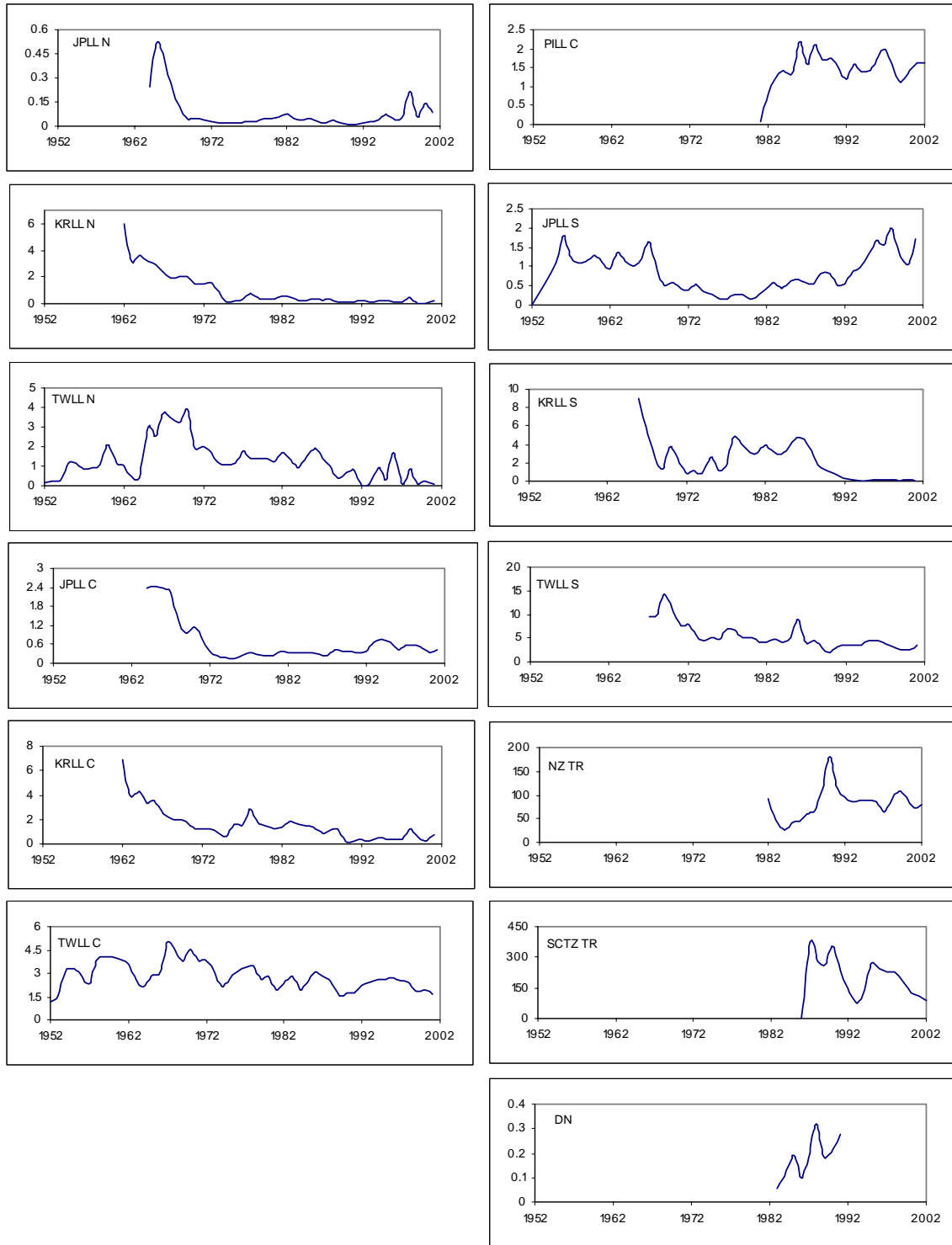
Figure 4. Catch per unit effort by fishery. Units are catch number per 100 hooks for the longline fisheries, catch number per boat/day for troll fisheries and tonnes per day for the driftnet fishery.
