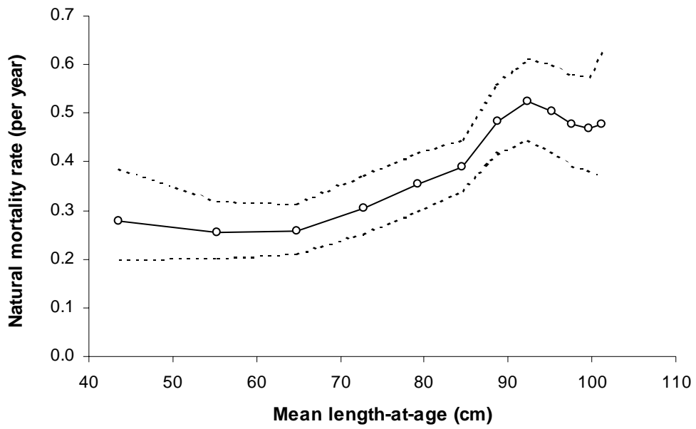
Figure 13. Estimated natural mortality rate by age-class plotted against mean length-at-age with 95% confidence intervals.
