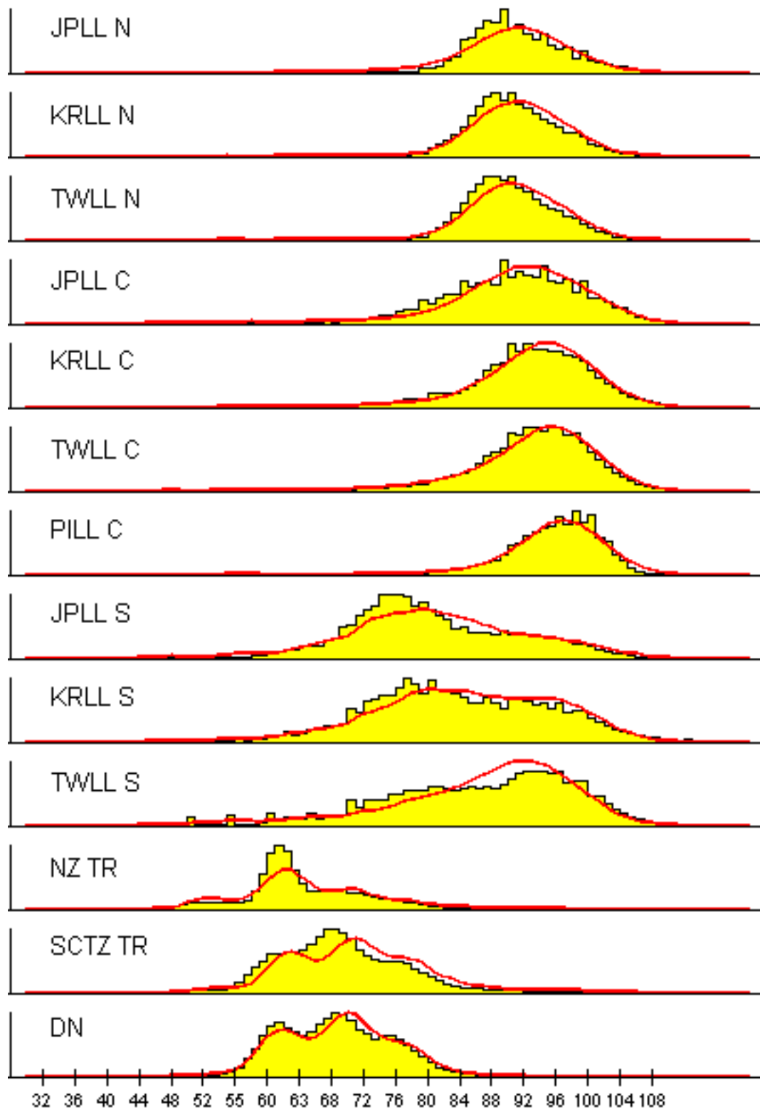
Figure 6. Observed (histograms) and predicted (line) length frequencies for each fishery aggregated over time.
