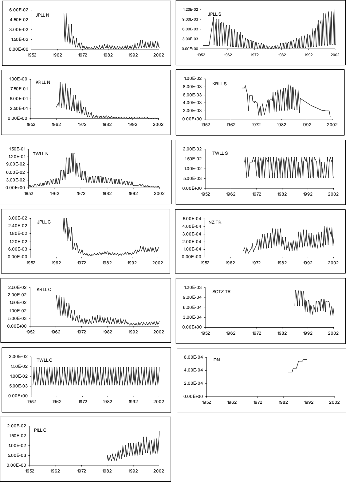
Figure 7. Time series of catchability coefficients by fishery.
