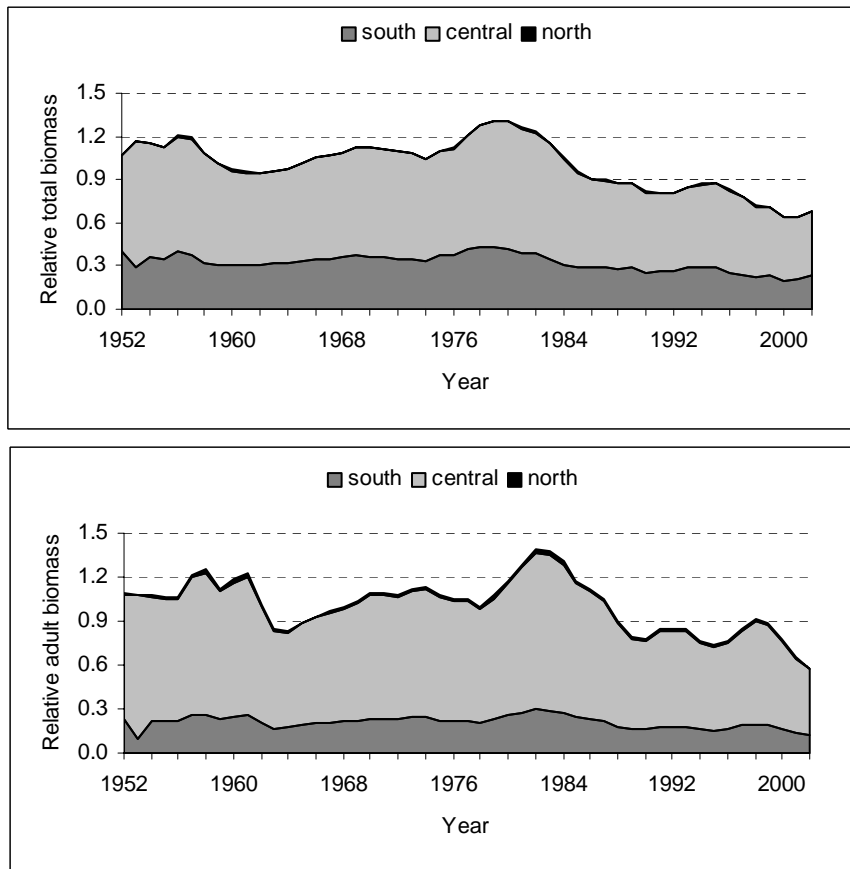
Figure 16. Estimates of relative total and adult biomass, by region.
