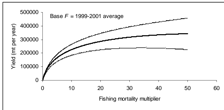
Figure 20. Predicted equilibrium yield and 95% confidence intervals as a function of fishing mortality (relative to the average fishing mortality-at-age during 1999-2001).
