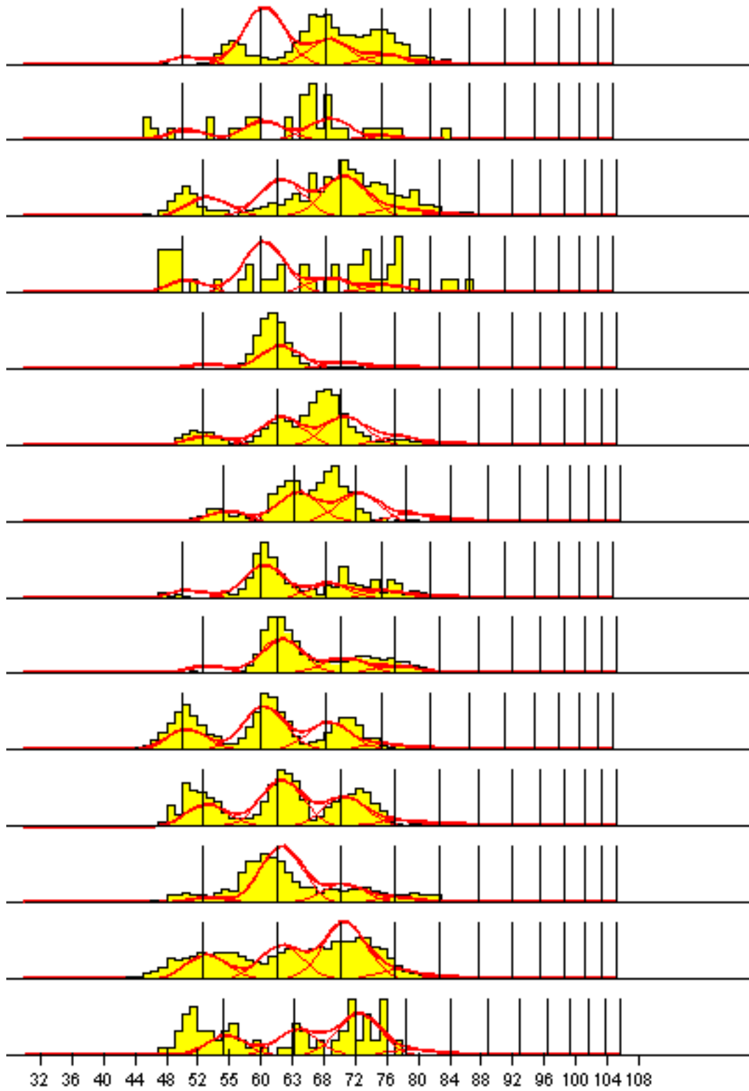
Figure 7. Observed (histograms) and predicted (line) length frequencies for the New Zealand domestic troll fishery for quarterly periods during 1989-2001. The vertical bars indicate the estimated mean lengths-at-age.
