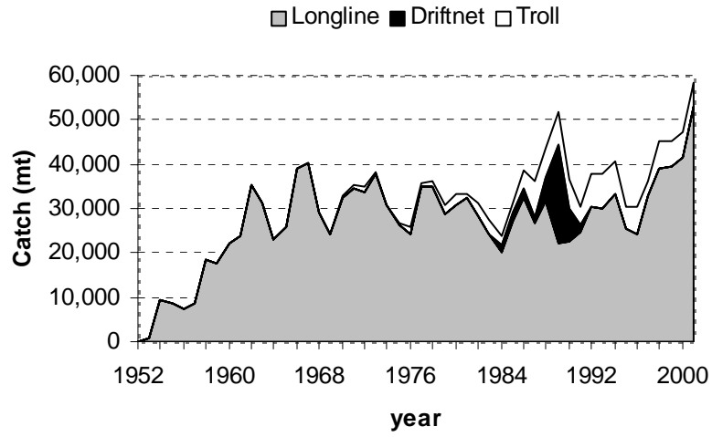
Figure 3. South Pacific albacore catch by gear type, 1952-2002.
