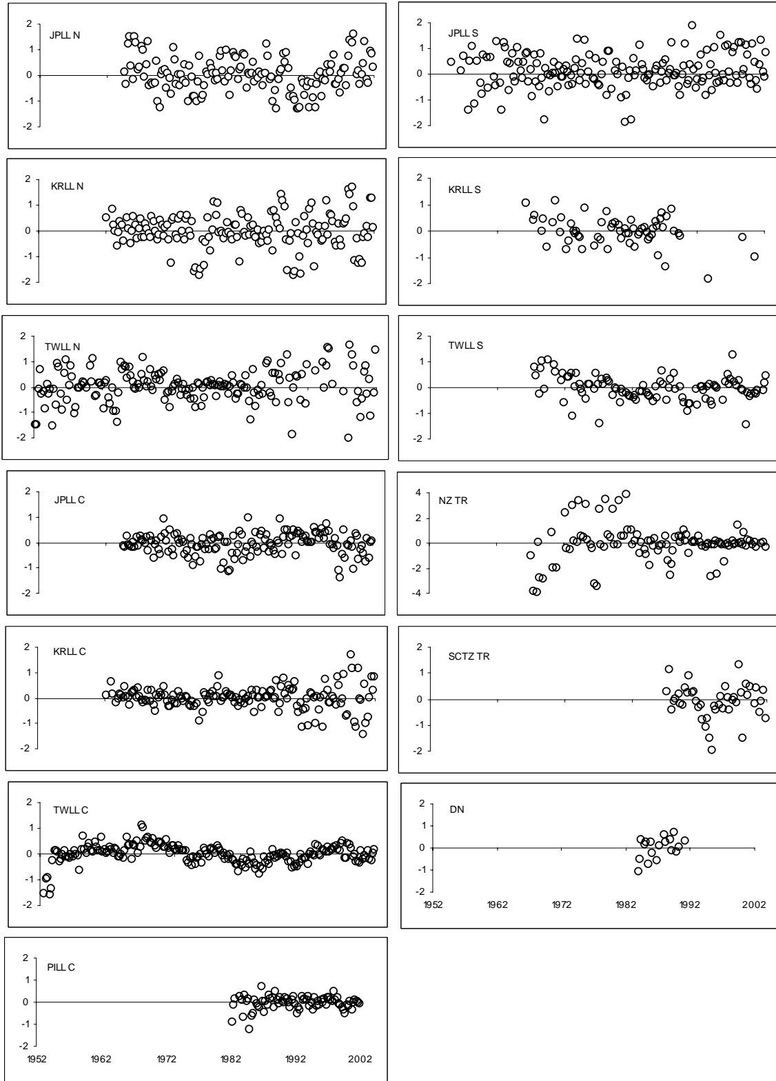
Figure 12. Effort deviations by fishery.
