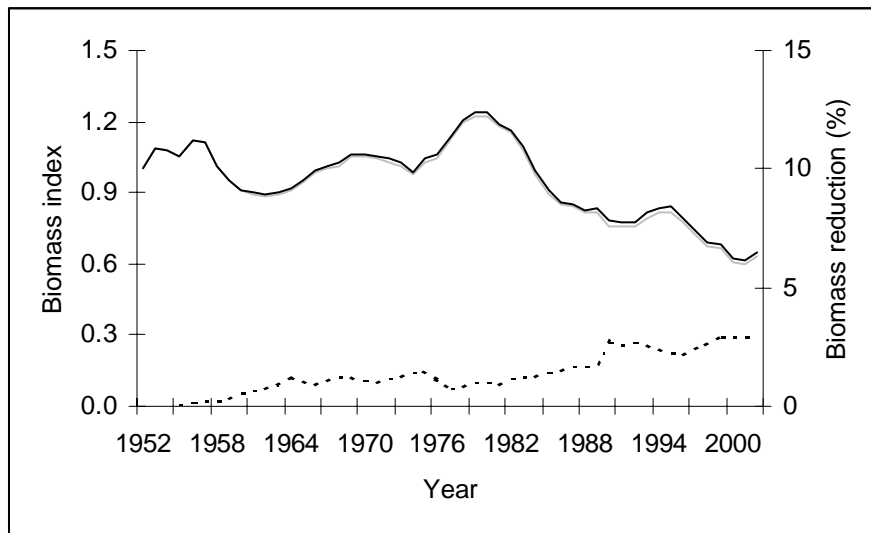
Figure 18. Comparison of the estimated biomass trajectory (upper thick line) with the biomass trajectory that would have occurred in the absence of fishing (upper thin line). The lower dotted line depicts the percentage difference between the two trajectories.
