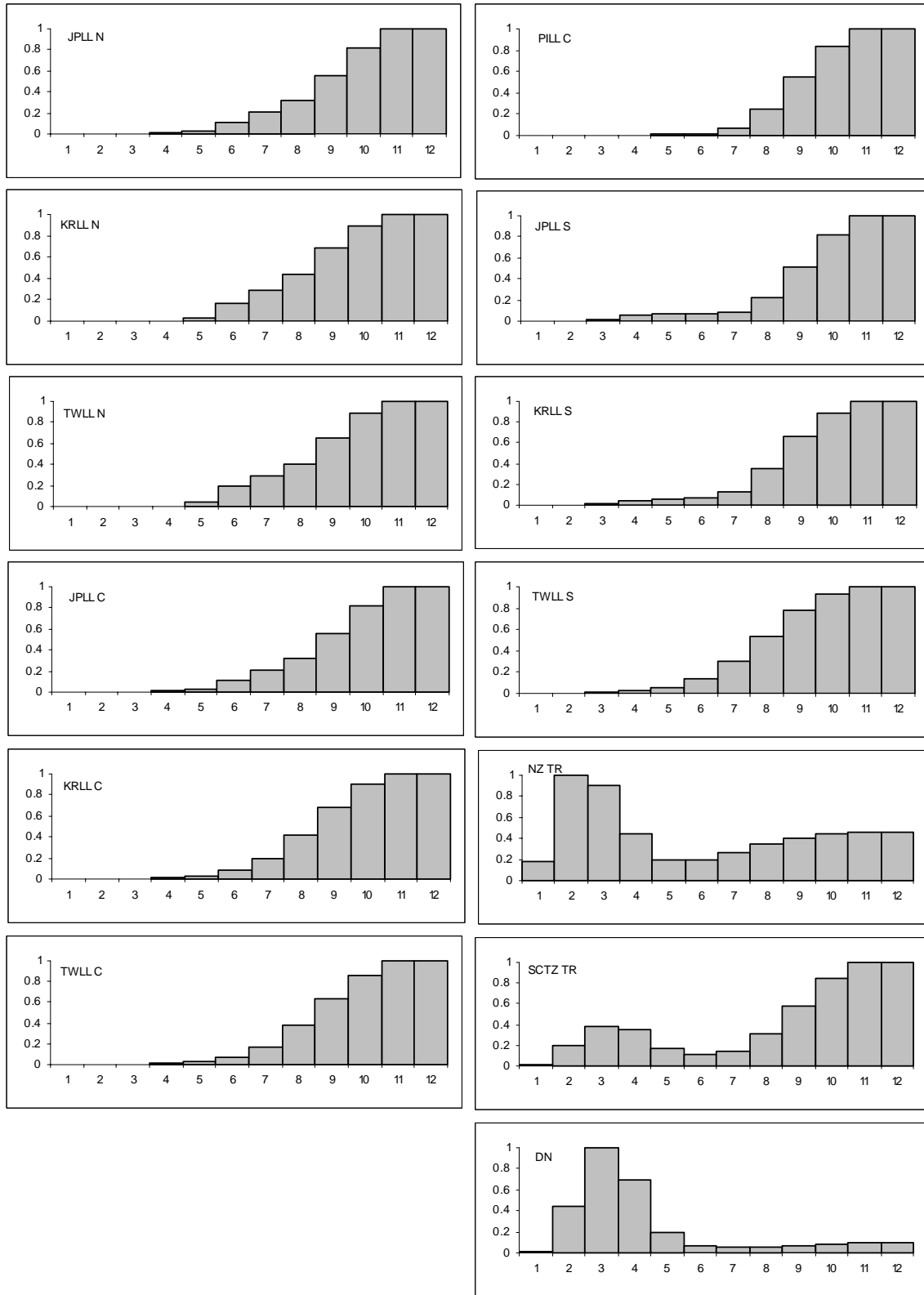
Figure 11. Selectivity coefficients, by fishery.
