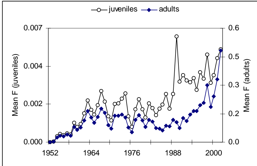
Figure 17. Estimated average annual fishing mortality rates for juvenile (ages 1-5) and adult (ages 6-12) albacore in the South Pacific.
