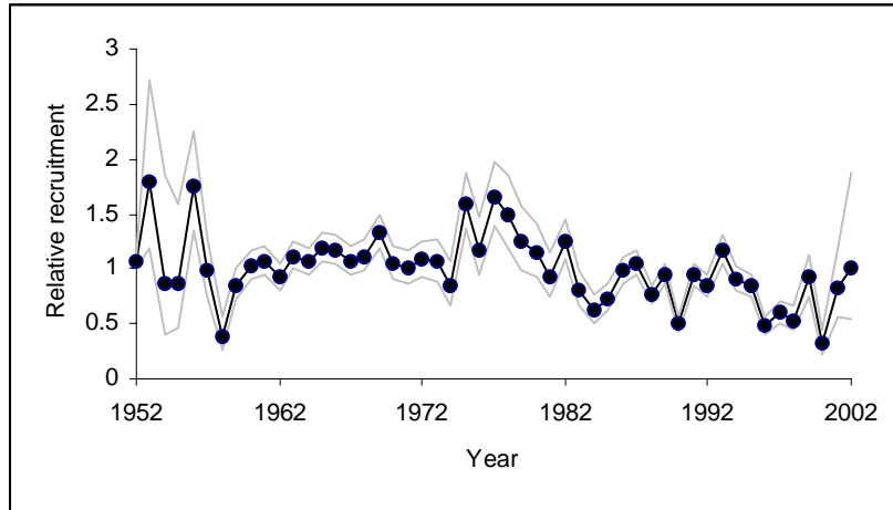
Figure 15. Estimated annual recruitment, with 95% confidence intervals, scaled to the average of the point estimates.
