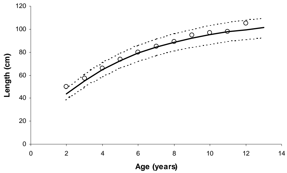
Figure 10. Estimated mean lengths-at-age (heavy line) and the variability of length-at-age (dotted lines represent \pm 2 SD) assuming that the first age class is two years of age. The circles are mean lengths corresponding to annuli on South Pacific albacore vertebrae (from Labelle et al. 1993).
