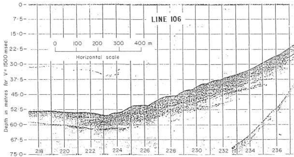
Figure 8. Hummocky topography between fixes 223-231 on the lower shelf slope adjacent to the Teae River indicating past downslope movement of sediment.
