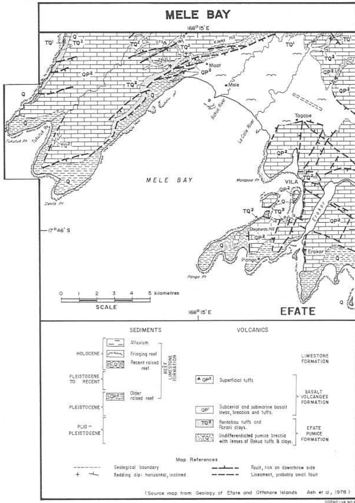
Figure 2. Geology of Mele Bay.
