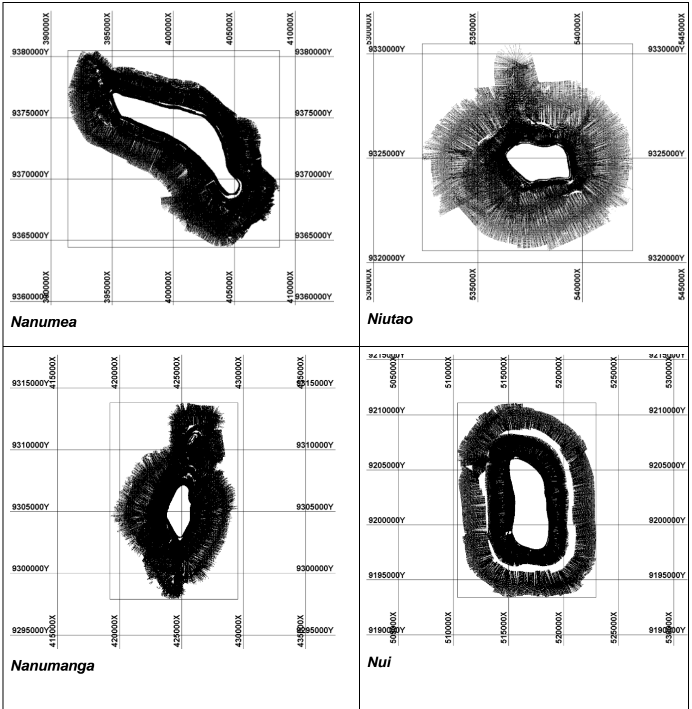
Appendix 1, Figure 28 – Multibeam Echosounder Coverage
