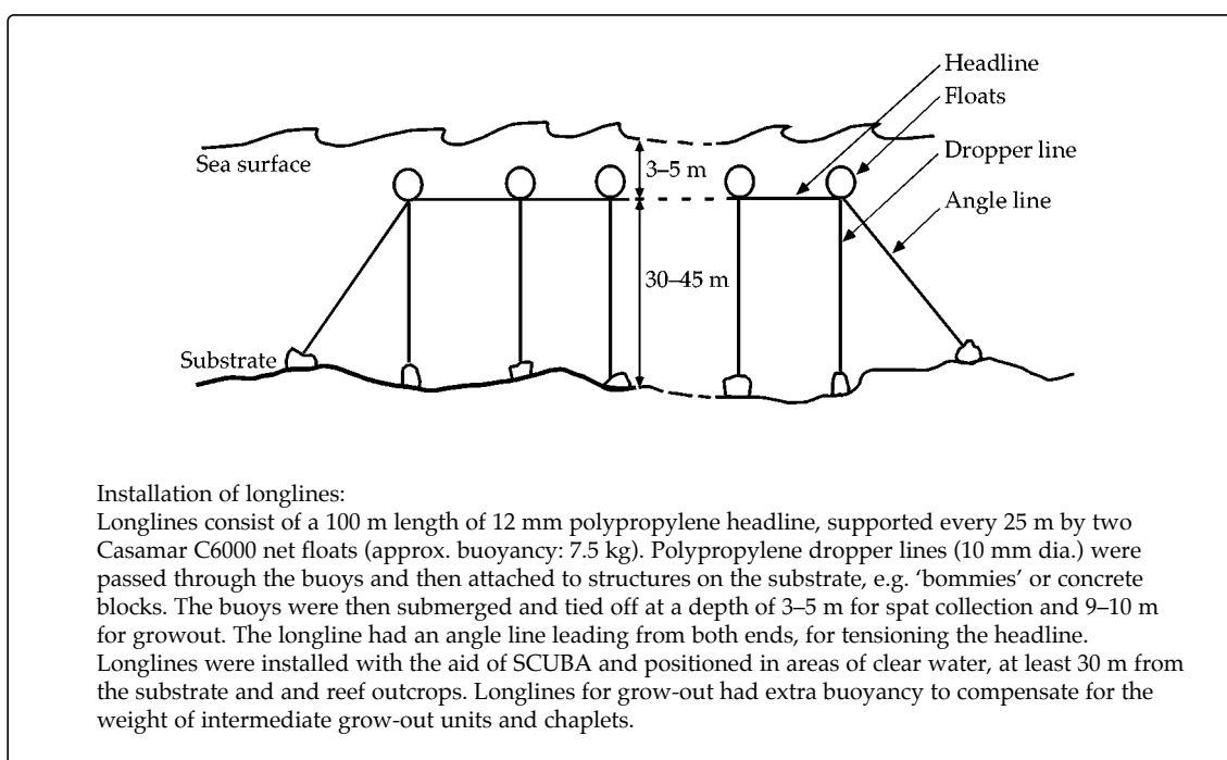
Figure 1: Diagram of longlines and methods used to install them
