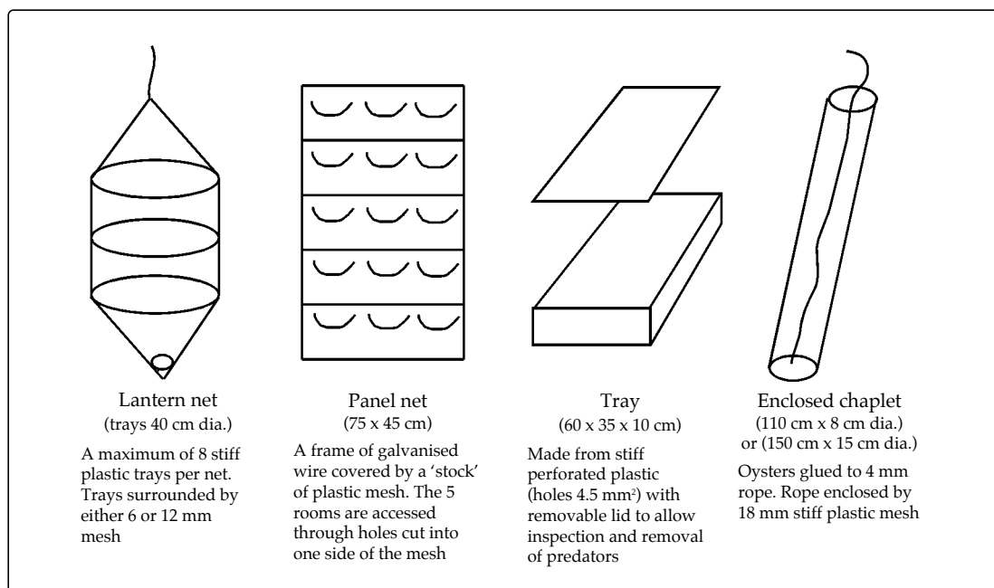
Figure 4: The intermediate culture systems used to grow out spat removed from collectors
