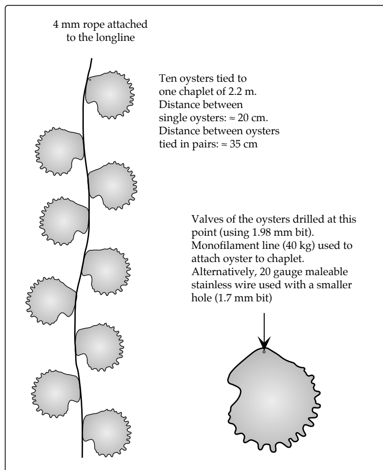
Figure 6: Chaplet system for growing out oysters and holding seeded stock
