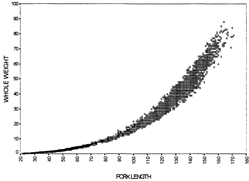
Figure 4. Yellowfin whole weight (kg) vs upper jaw to caudal fork length (cm) for yellowfin, with outliers removed
