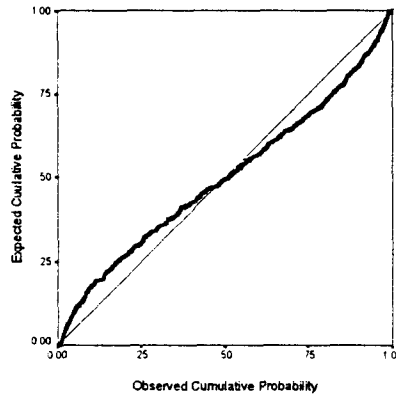
Figure 1. Normal probability plot for regression of logarithm of yellowfin fork length on logarithm of whole weight, with presence of outliers
