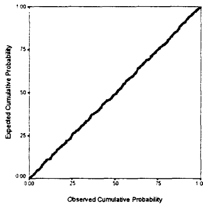
Figure 2. Normal probability plot for regression of logarithm of yellowfin fork length on logarithm of whole weight, with outliers removed
