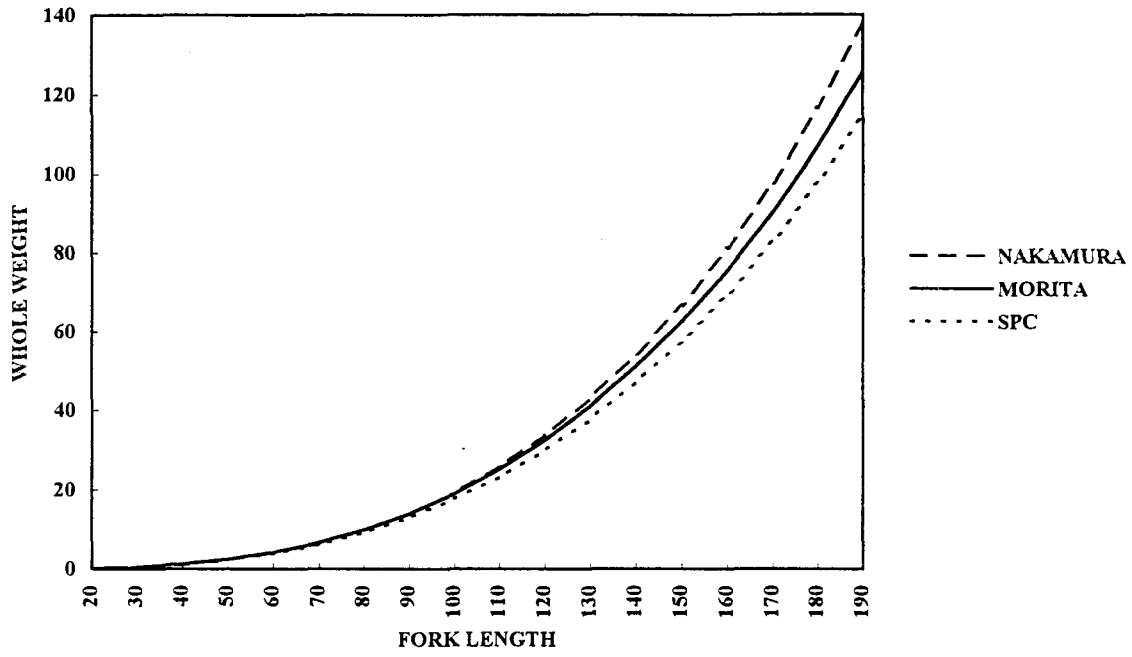
Figure 6. Fitted yellowfin whole weight (kg) – fork length (cm) curves from Nakamura & Uchiyama (1966), Morita (1973), and SPC data
