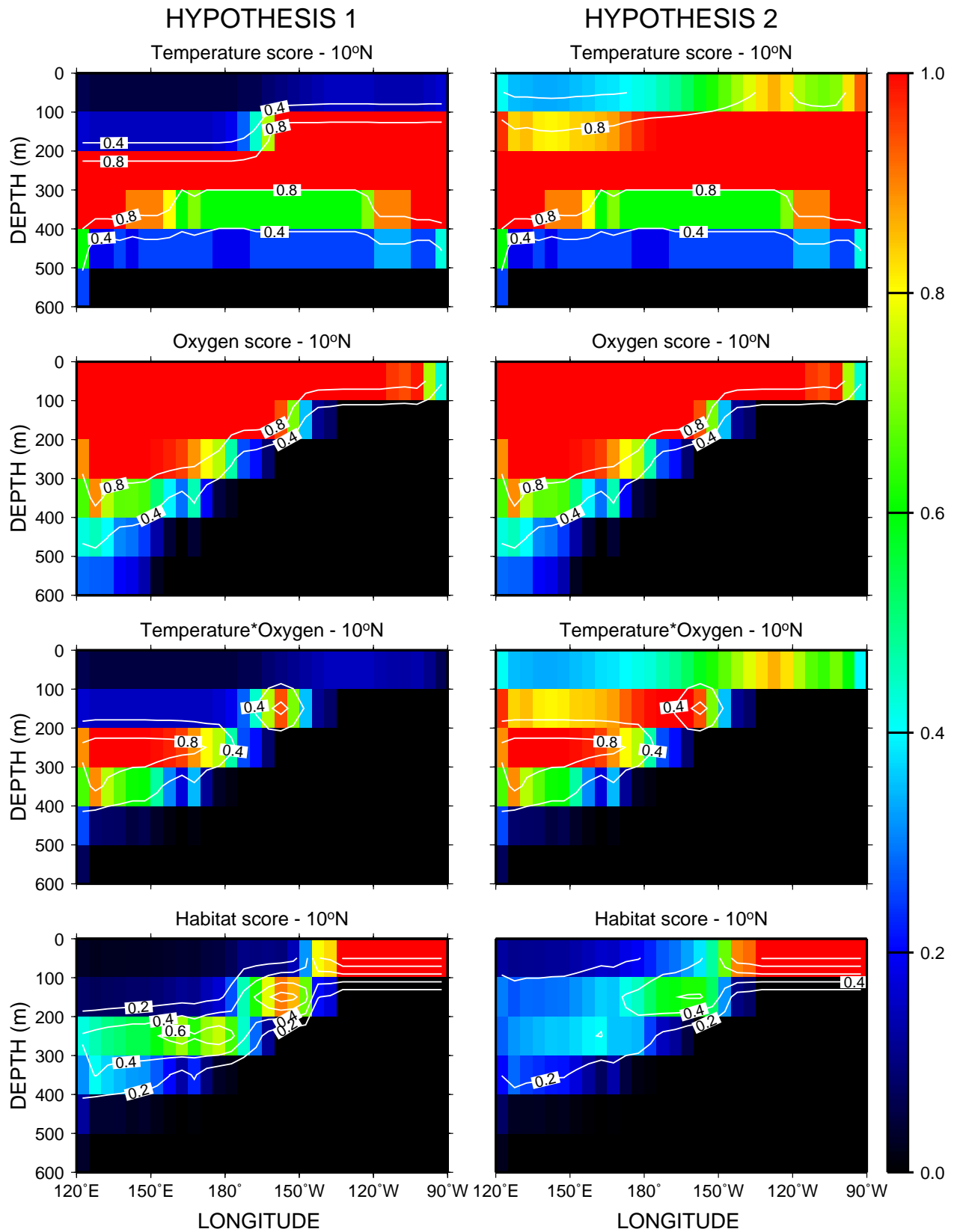
Figure 30. Zonal section at 10°N of climatological bigeye tuna habitat indices for temperature, oxygen, combined temperature and oxygen and normalised habitat quality ( p_{jky} ). Habitat indices follow hypothesis 1 (left) or hypothesis 2 (right).
