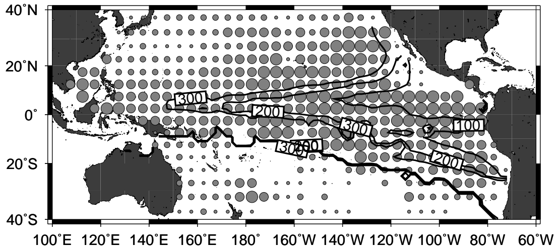
Figure 24. Relationship between the annual depth distribution of the 2 ml l -1 DO isopleth and nominal bigeye CPUE for the Japanese longline fleet (1986-95). Only the 100 to 300 m depths are illustrated.
