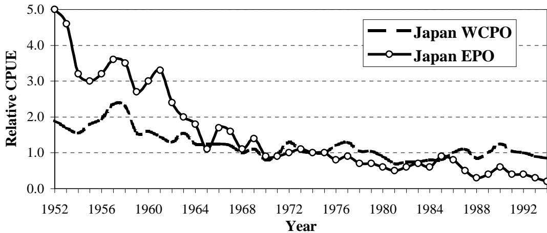
Figure 25. Standardised Japanese longline CPUE for the western and central (WCPO) and eastern Pacific Ocean (EPO) after Miyabe (1995).
