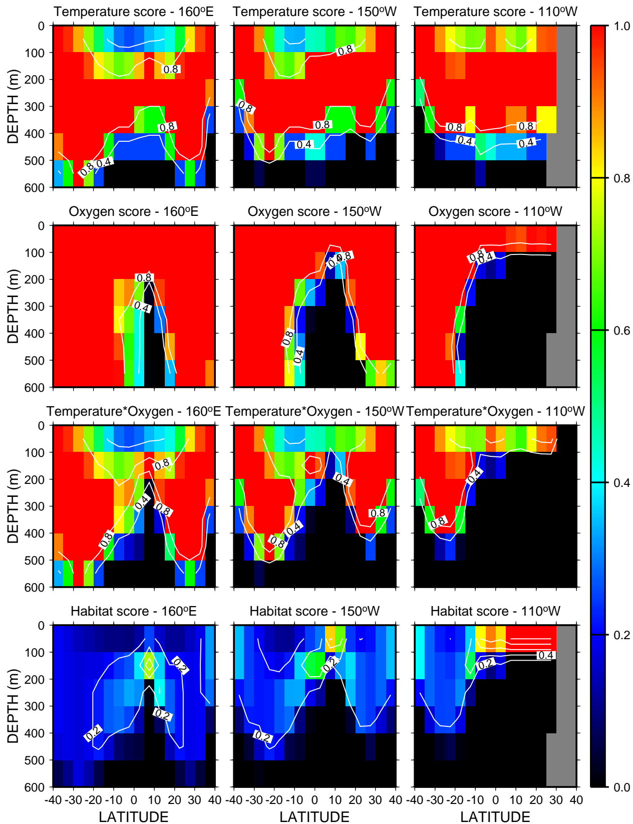
Figure 29. Meridional sections (160°E, 150°W and 110°W) of climatological bigeye tuna habitat indices for temperature, oxygen, combined temperature and oxygen and normalised habitat quality ( p_{jky} ). Habitat indices follow hypothesis 2.
