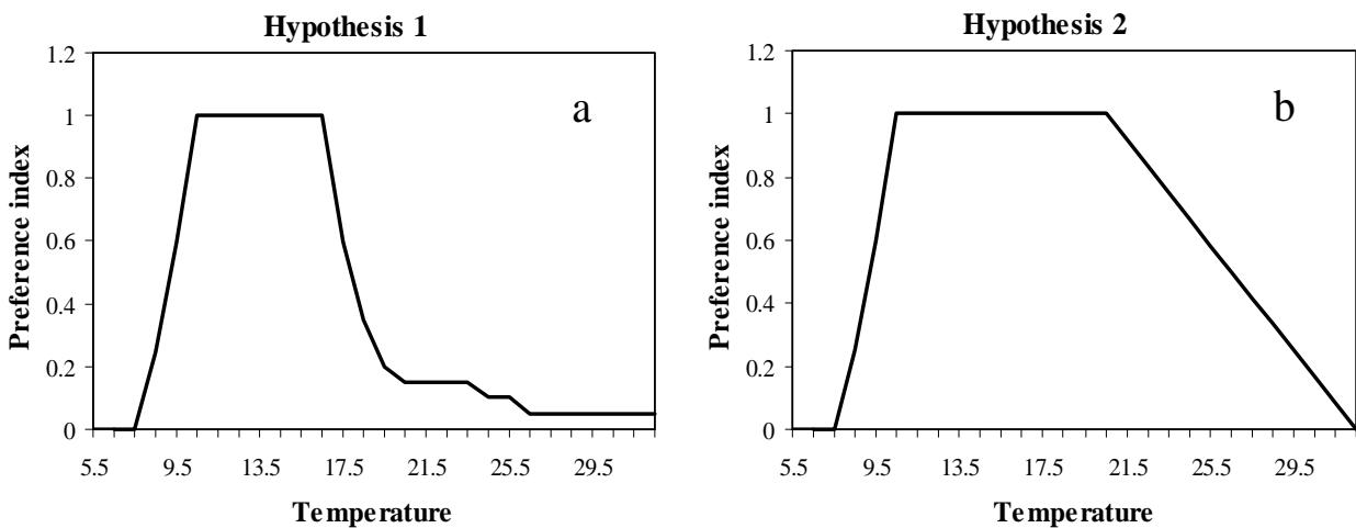
Figure 26. Alternative hypotheses regarding temperature preferences of bigeye tuna: (a) based on sonic tracking (Holland et al., 1990) and longline TDR observations (Boggs, 1992) and (b) assuming a stronger preference for water temperatures > 17°C.
