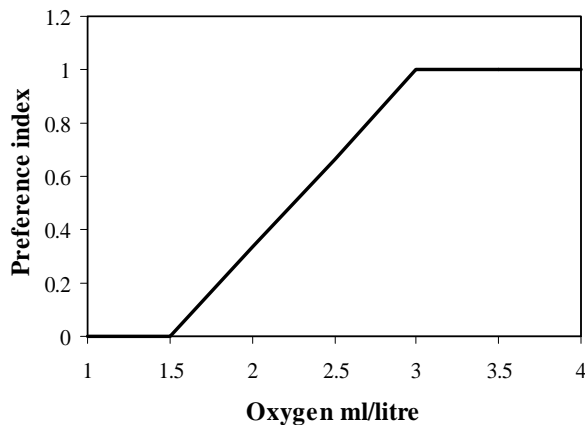
Figure 27. Dissolved oxygen preference of bigeye tuna, based on various physiological observations.
