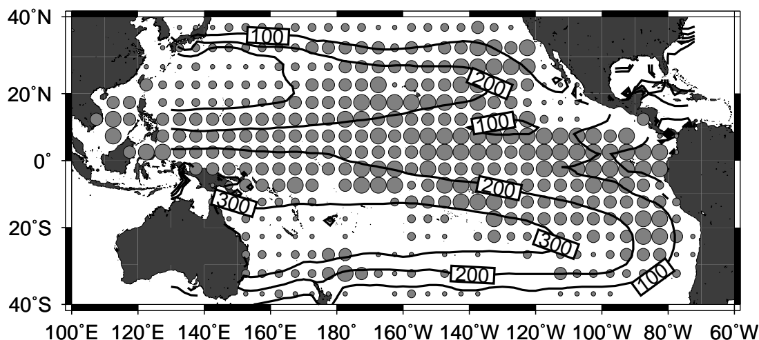
Figure 23. Relationship between the annual depth distribution of 15°C isotherm and nominal bigeye CPUE for the Japanese longline fleet (1986–95).
