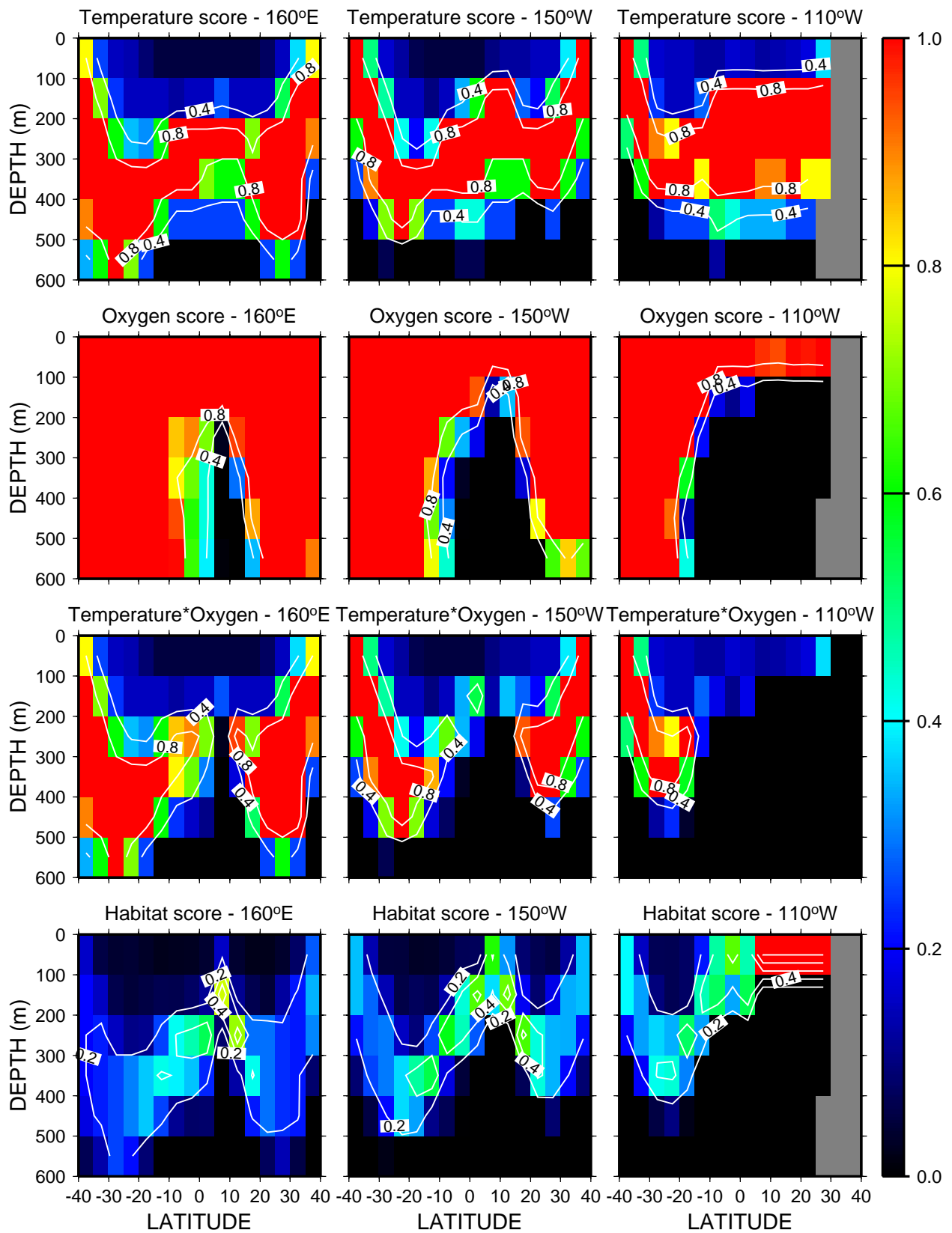
Figure 28. Meridional sections (160°E, 150°W and 110°W) of climatological bigeye tuna habitat indices for temperature, oxygen, combined temperature and oxygen and normalised habitat quality ( p_{jky} ). Habitat indices follow hypothesis 1.
